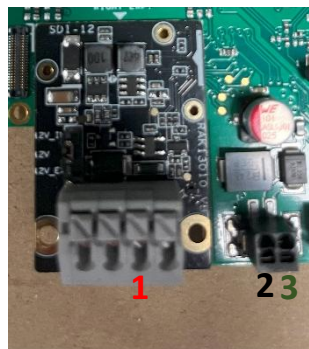
Figure 29: SDI12 module to data logger connections: 1 - DATA, 2 - GND, 3 – 12V
